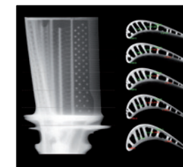
Turbine blade
